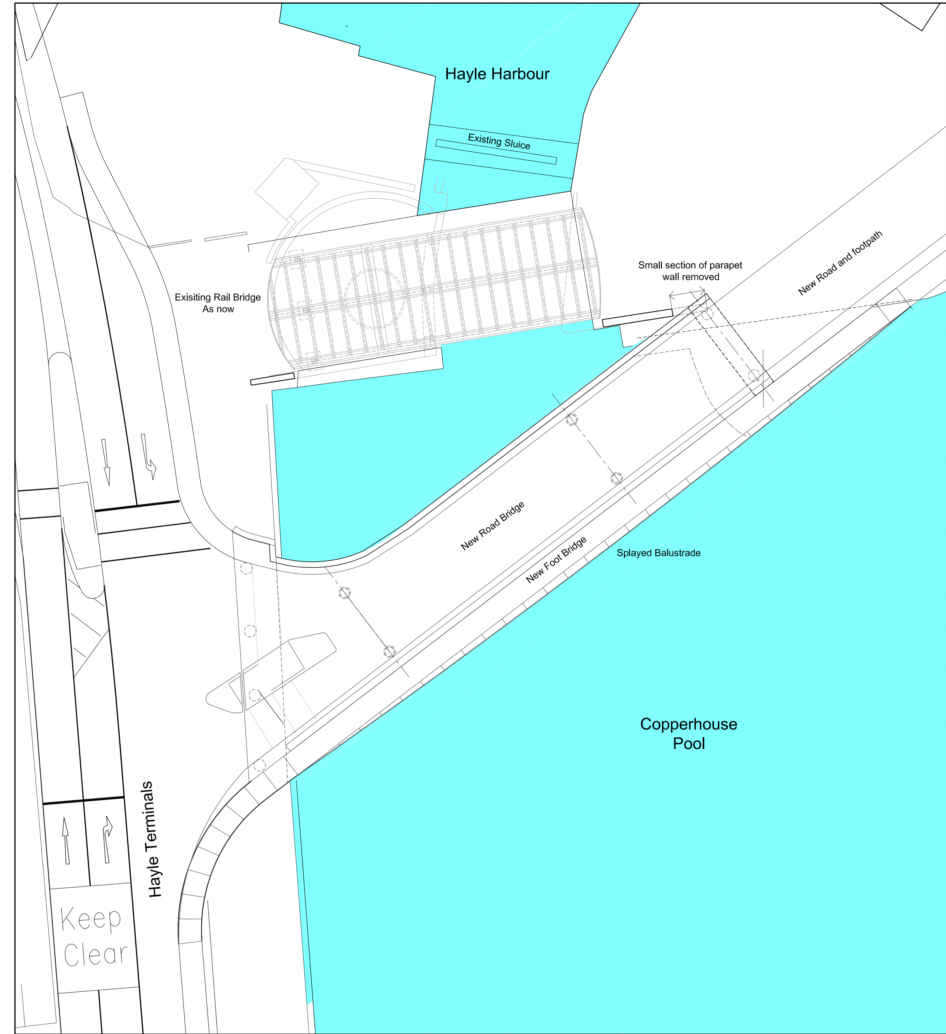
Proposed Plan Scale 1:200
